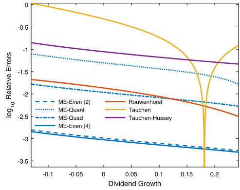
(b) \rho = 0.9, \gamma = 1.5, N = 15.
